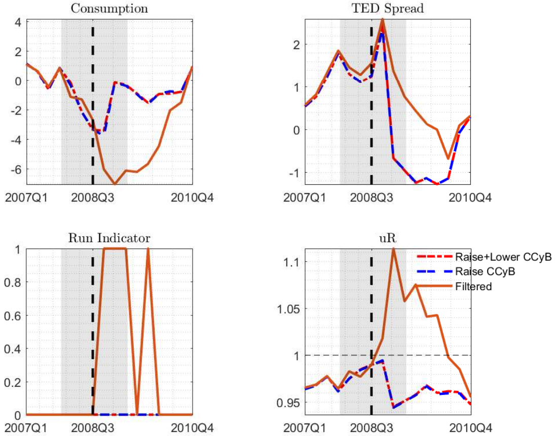
Figure 11: Estimated series (orange solid line) vs. counterfactual where regulator raises capital requirements before the crisis (dashed blue line), and counterfactual where regulator can both raise and lower capital requirements (dotted red line)
