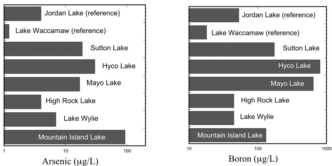
Fig. 7. Concentrations of arsenic and boron in pore water from lakes located near CCR storage sites (Sutton, Hyco, Mayo, High Rock, Wylie, and Mountain Island (Brandt, 2018; Ruhl et al., 2012) compared to reference lakes without potential impact from nearby CCR storage sites (Waccamaw and Jordan). The location of the lakes is shown in Fig. 1. The enrichment of As and B in pore water from bottom sediments in lakes located nearby CCR storage sites is suggested to be derived from mobilization of As and B from CCR solids that were spilled and accumulated in the lakes, as evidenced by the Sutton Lake case.
