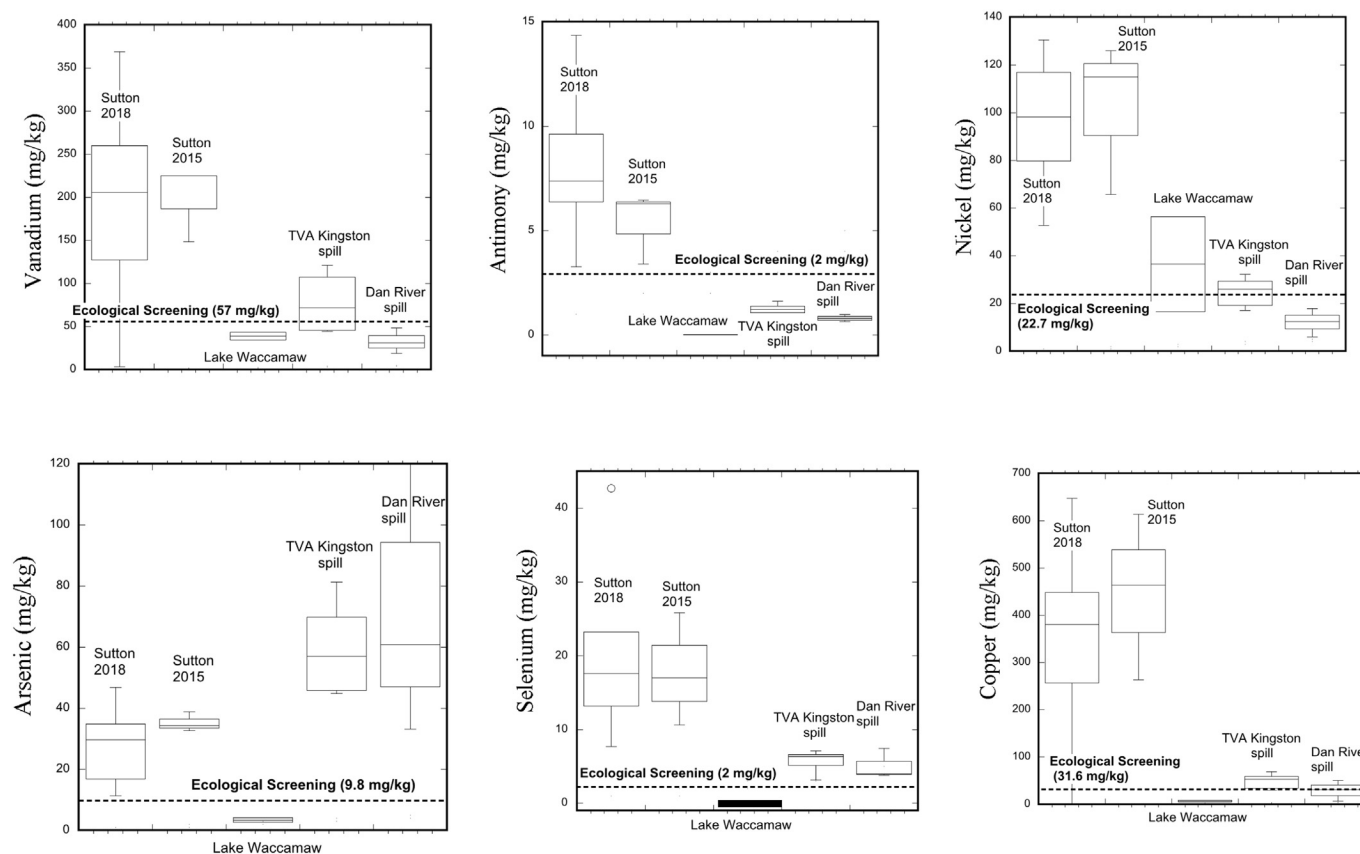
Fig. 6. Box plots of selected metals with ecological impact measured in sediments collected from Sutton Lake in 2018 and 2015, Lake Waccamaw (reference lake), and in sediments impacted by the TVA Kingston (Tetra Tech Inc, 2008) and Dan River (North Carolina Department of Environment and Natural Resources, 2018) coal ash spills, compared to freshwater sediment screening benchmarks values for sediment toxicity used by U.S. EPA (MacDonald et al., 2000; MacDonald et al., 2003). Results from Sutton Lake sediments show high levels of metals, which are comparable, and in most cases higher, than concentrations found in sediments impacted by the TVA Kingston and Dan River coal ash spills. The metal concentrations exceeded the acceptable screening thresholds for aquatic freshwater sediment toxicity used by U.S. EPA to define potential ecological impact (Long et al., 2000, 2006; MacDonald et al., 2000; MacDonald et al., 2003).
