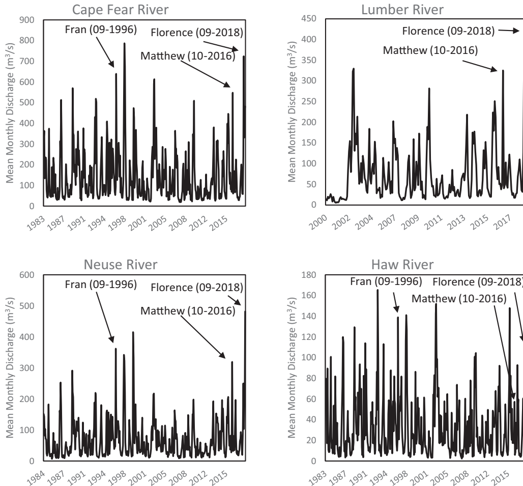
Fig. 5. Hydrographs of mean monthly discharge rates ( \text{m}^3/\text{s} ) of major river systems in North Carolina (see locations in Fig. 1). Data was generated from U.S. Geological Survey Current Water Data for North Carolina (2018).
