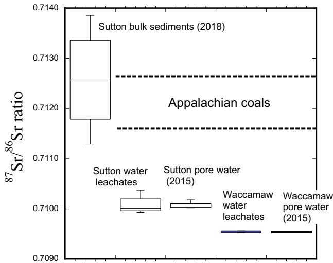
Fig. 4. Box plot of Sr isotope variations in Sutton Lake sediments, water leachates extracted from Sutton Lake sediments, Sutton pore water collected in 2015, Waccamaw Lake sediments, and Waccamaw pore water collected in 2015. The Sr isotope data indicate that (1) sediments from Sutton Lake have a ^{87}\text{Sr}/^{86}\text{Sr} ratio that mimic the ratios reported for the Appalachian coals (Vengosh et al., 2013); and (2) that Sr isotope ratios in water leachates are identical to corresponding pore water in both the Sutton and Waccamaw lakes; and (3) selective mobilization of Sr to the water phase with a lower ^{87}\text{Sr}/^{86}\text{Sr} ratio relative to the ^{87}\text{Sr}/^{86}\text{Sr} in the bulk sediments. Sr isotope ratios in Sutton Lake and Lake Waccamaw pore waters from 2015 are from Brandt et al. (2018).
